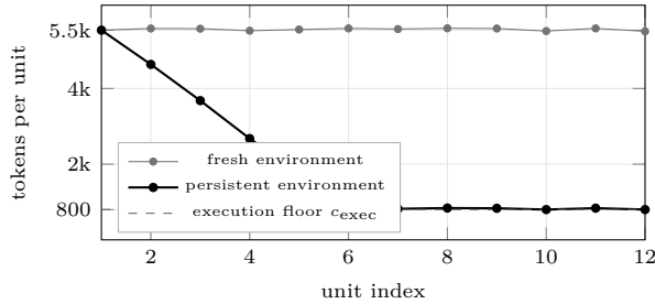
Figure 2: E3, harness output (mock mode): cost per unit across twelve similar units. Persistent memory decays 85.6% to the floor; fresh context pays cold start every time. The scripted agent implements Equation (8), so this is a consistency demonstration; real-mode measurement is in progress.
